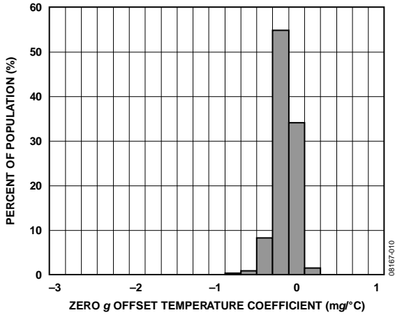
Figure 10. X-Axis Zero g Offset Temperature Coefficient, V_S = 2.6\text{ V}
