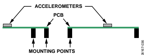
Figure 44. Incorrectly Placed Accelerometers
