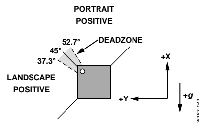
Figure 50. Orientation Showing a 15.4° Dead Zone Region
