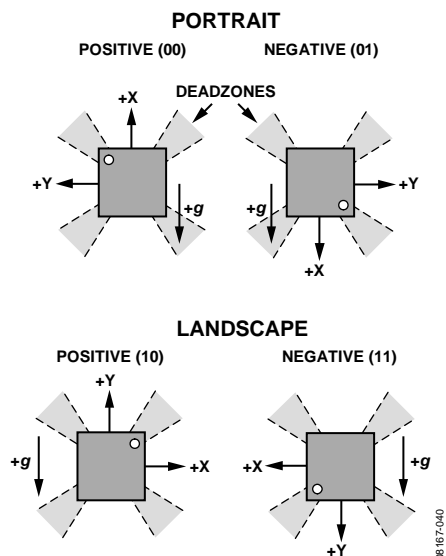
Figure 49. 2D Orientation with Corresponding Codes
