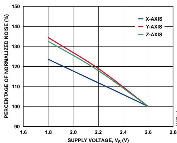
Figure 55. Normalized Noise vs. Supply Voltage
