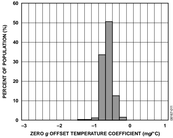
Figure 11. Y-Axis Zero g Offset Temperature Coefficient, V_S = 2.6\text{ V}
